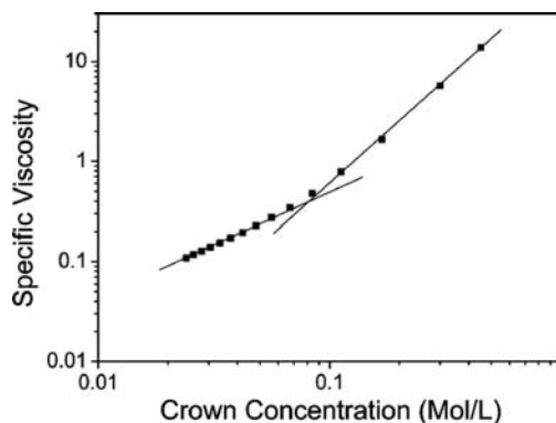
Figure 22. Specific viscosity of acetone solutions of equimolar mixtures of 87 and 88 as a function of the total concentration. (Reprinted from ref 243. Copyright 2007 American Chemical Society.)
