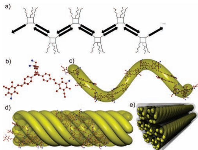
Figure 38. Mode of polymerization and hierarchical supramolecular organization of the merocyanine dyes. (Reprinted with permission from ref 416 Copyright 2003 John Wiley & Sons, Inc.)
