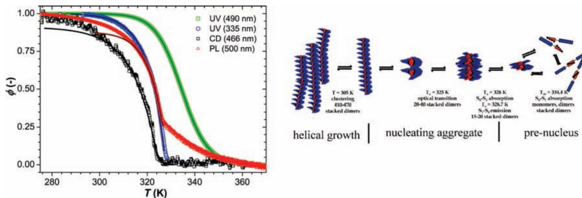
Figure 40. Degree of aggregation, \phi , based on UV-vis, CD, and PL spectroscopy for 133 and the schematic representation of the supramolecular polymerization of 132–134 . (Reprinted with permission from ref 324. Copyright 2006 American Association for the Advancement of Science.)
