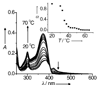
Figure 42. Temperature-dependent UV-vis absorption for 154 in dodecane ( 1.1 \times 10^{-5} M). (Inset) Fraction of polymerized material, \alpha , versus temperature, as derived from the absorption at 380 nm. (Reprinted with permission from ref 443. Copyright 2006 John Wiley & Sons, Inc.)
